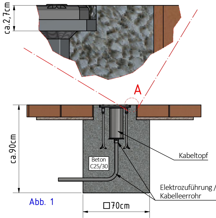
A (1:2)
