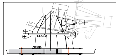
Klappadapter
